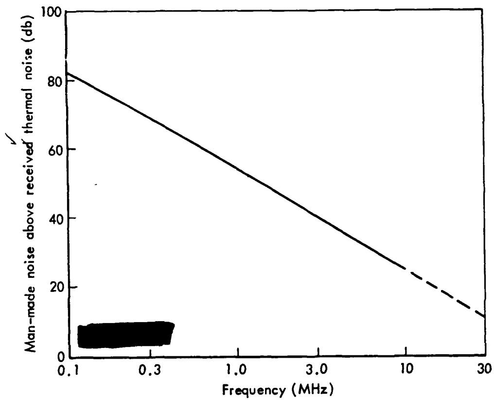
Fig. 5-3 CCIR quiet man-made noise levels (Ref. 2)
